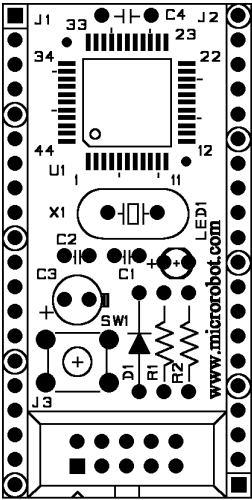
Fig 1.1 MR-16 CPU board silkscreen.
